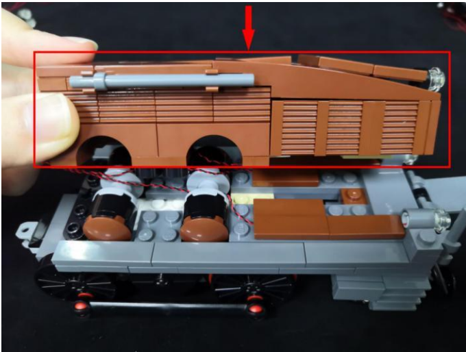
Take the Round Coin Cell Battery Pack, the expansion board, assemble them as per below, connect the cables of the lights to the expansion board, turn the power on to verify the lights.
